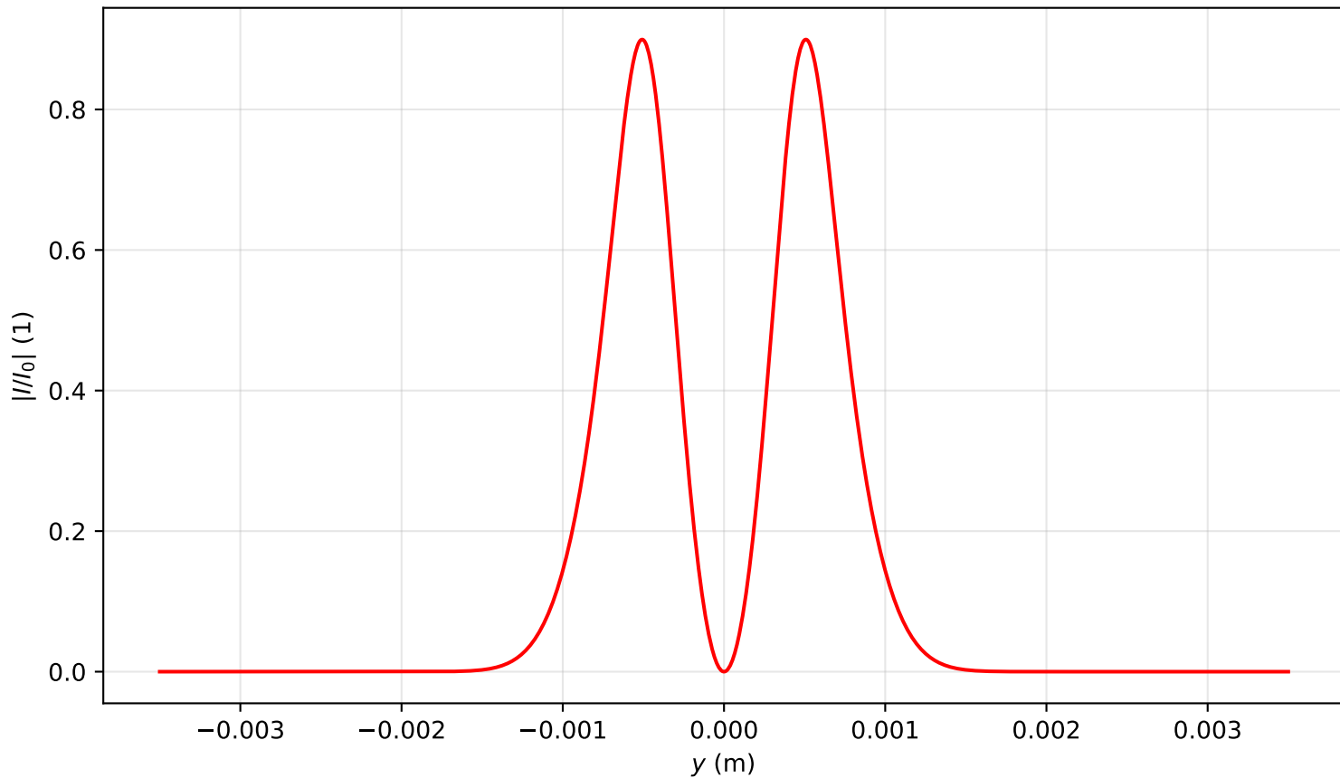
Intensity profile I(x=0, y, z=0.398)/I_0 , \text{Pin}=3.0\text{Pcr} , artificial time
